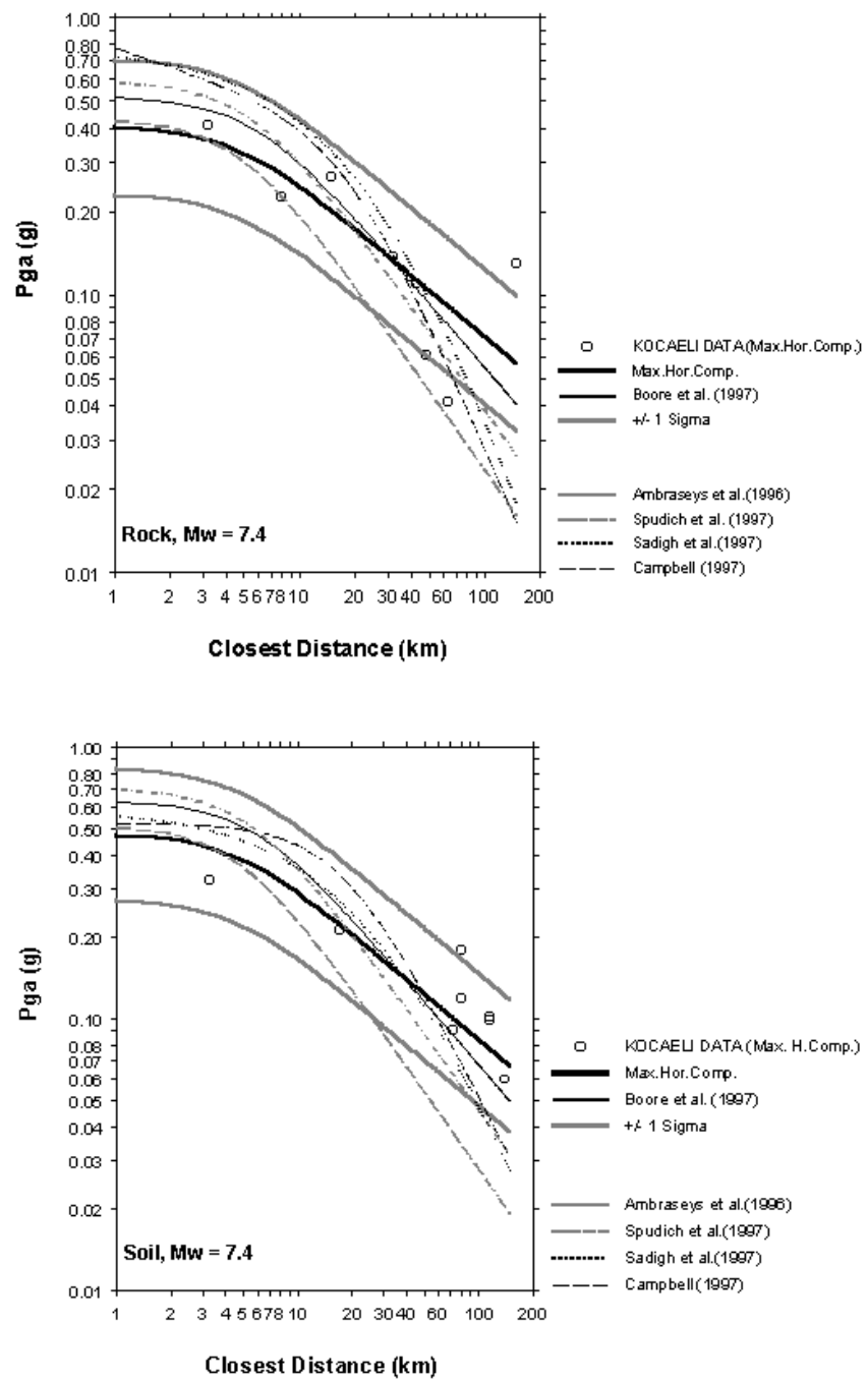
Figure 7. Curves of peak acceleration versus distance for magnitude 7.4 earthquake at rock and soil sites.
