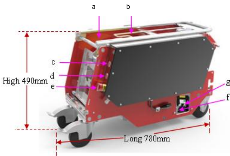
Side view of Motorized Cable Drum
